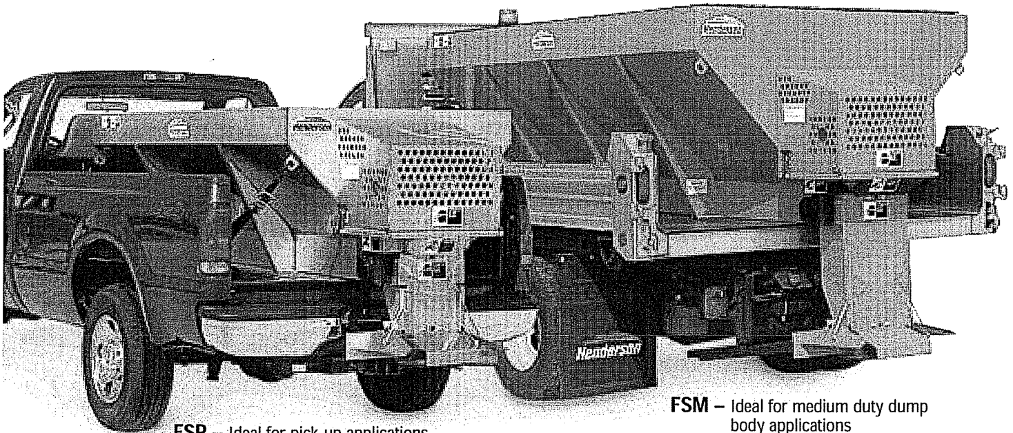
FSP – Ideal for pick-up applications
