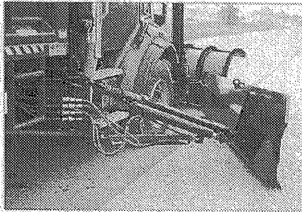
Wing in Flow position
