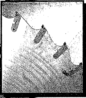
Replaceable Tips 24" and 48" Blades
