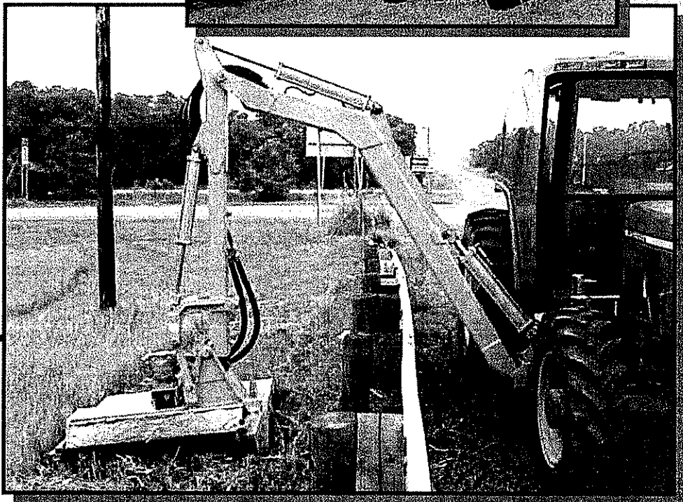
DB50 - 20' Boom - 50" Rotary Easily Reach Over Guard Rail or Other Obstacles
