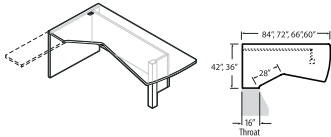
Extended Corner Island - RIGHT Recessed Modesty and Post
