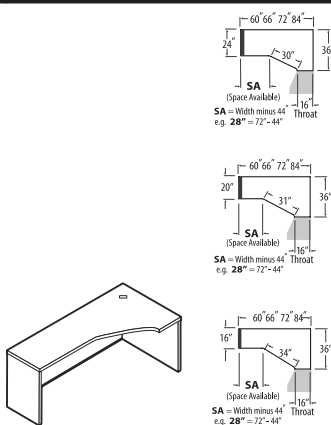
Right Extended Corner, 16" Throat
