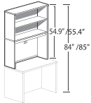
Open Hutch with Closed Back 54.9\"/>55.4\"/> High
