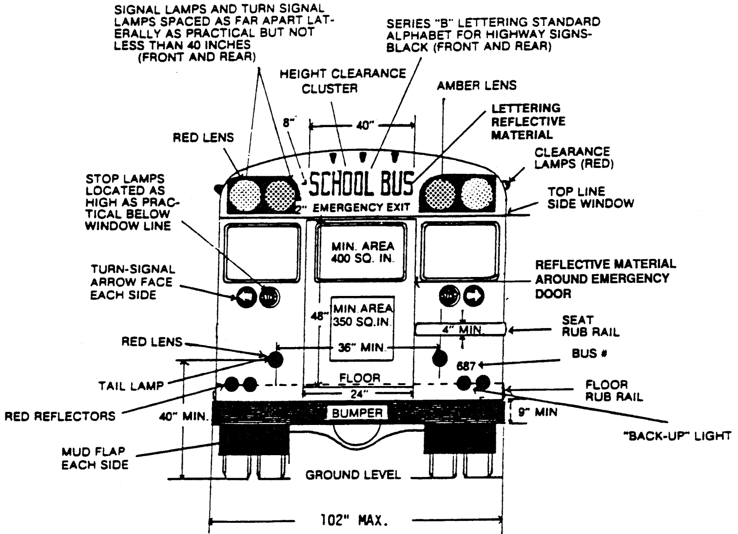
REAR ELEVATION
