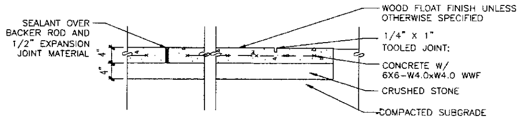
EXPANSION JOINT SEALANT DETAIL - N.T.S.
