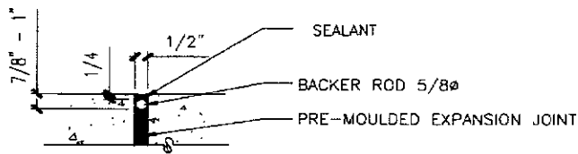
EXPANSION JOINT SEALANT DETAIL - N.T.S.
