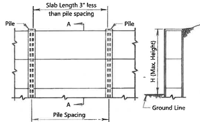
ELEVATION OF WALL
