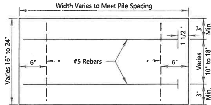
ELEVATION VIEW
