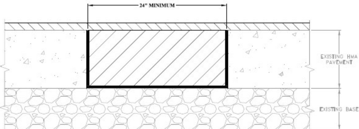
FULL DEPTH CRACK REPAIR IN FLEXIBLE PAVEMENT
