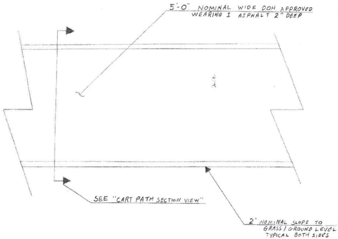
PAVING – PLAN VIEW
