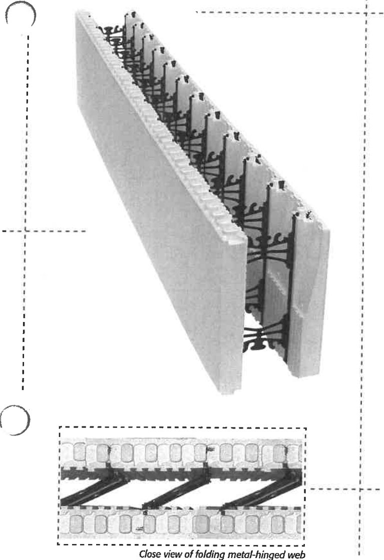
Close view of folding metal-hinged web
