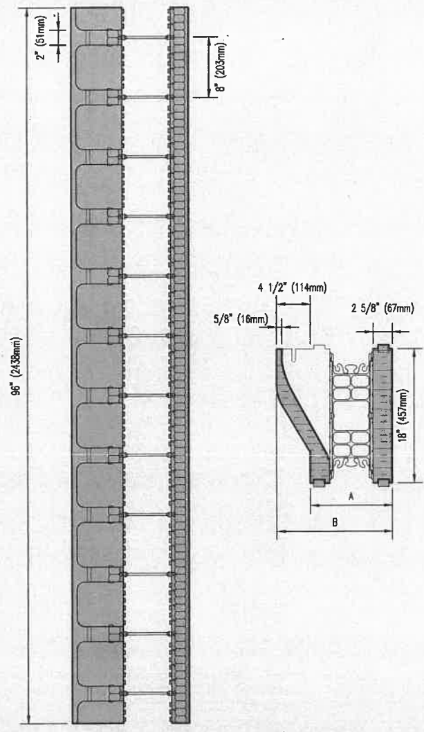
Unassembled 96" (2438mm) Molded Brick Ledge Shown Above
