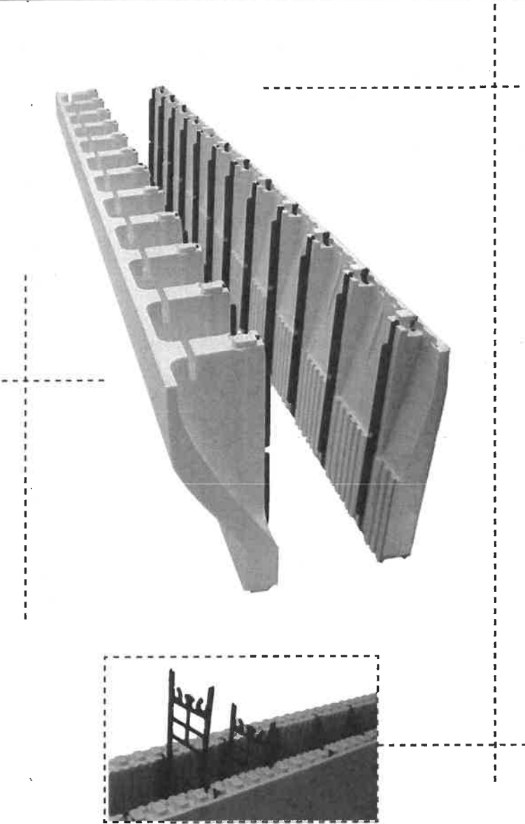
Close view of insert webs - available in 4"-12" (100-300mm) sizes
