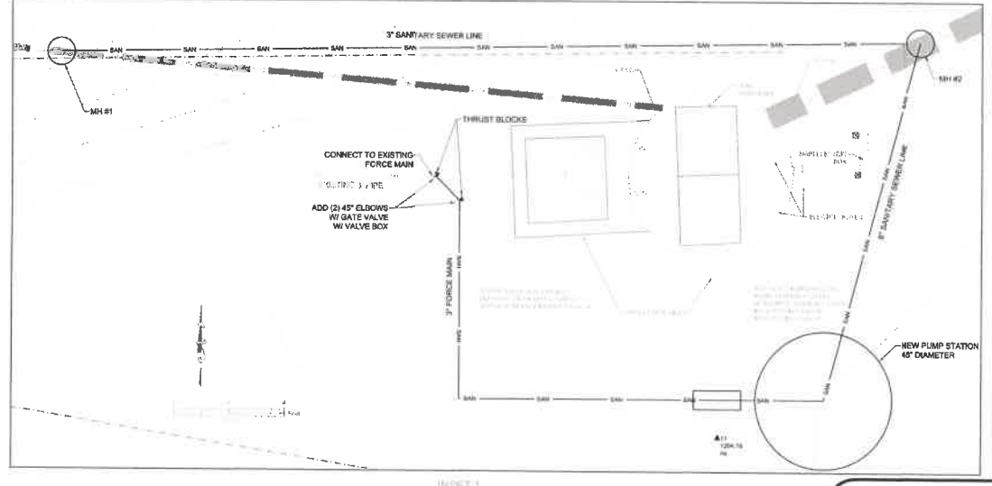
INSET 1 - EXISTING PUMP STATION BELOW LODGE
