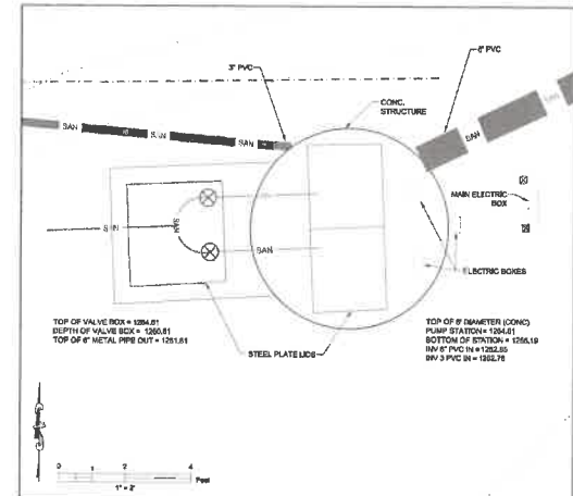
INSET 1 EXISTING PUMP STATION BELOW LODGE
