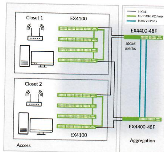
Figure 1: EX4100 Virtual Chassis configuration interconnected via dedicated front-panel 25GbE ports
