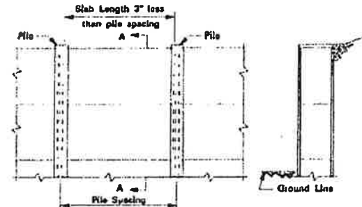
ELEVATION OF WALL
