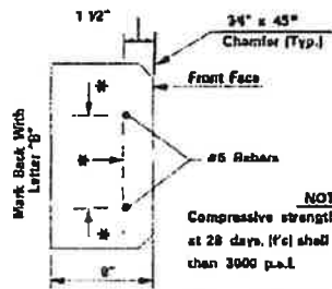
END VIEW
