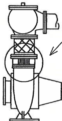
6" Triple Duty Valve and Flexible Connector, Shown Connected to 5" End Suction Pump Discharge with 6050 FLANGE ADAPTER.
