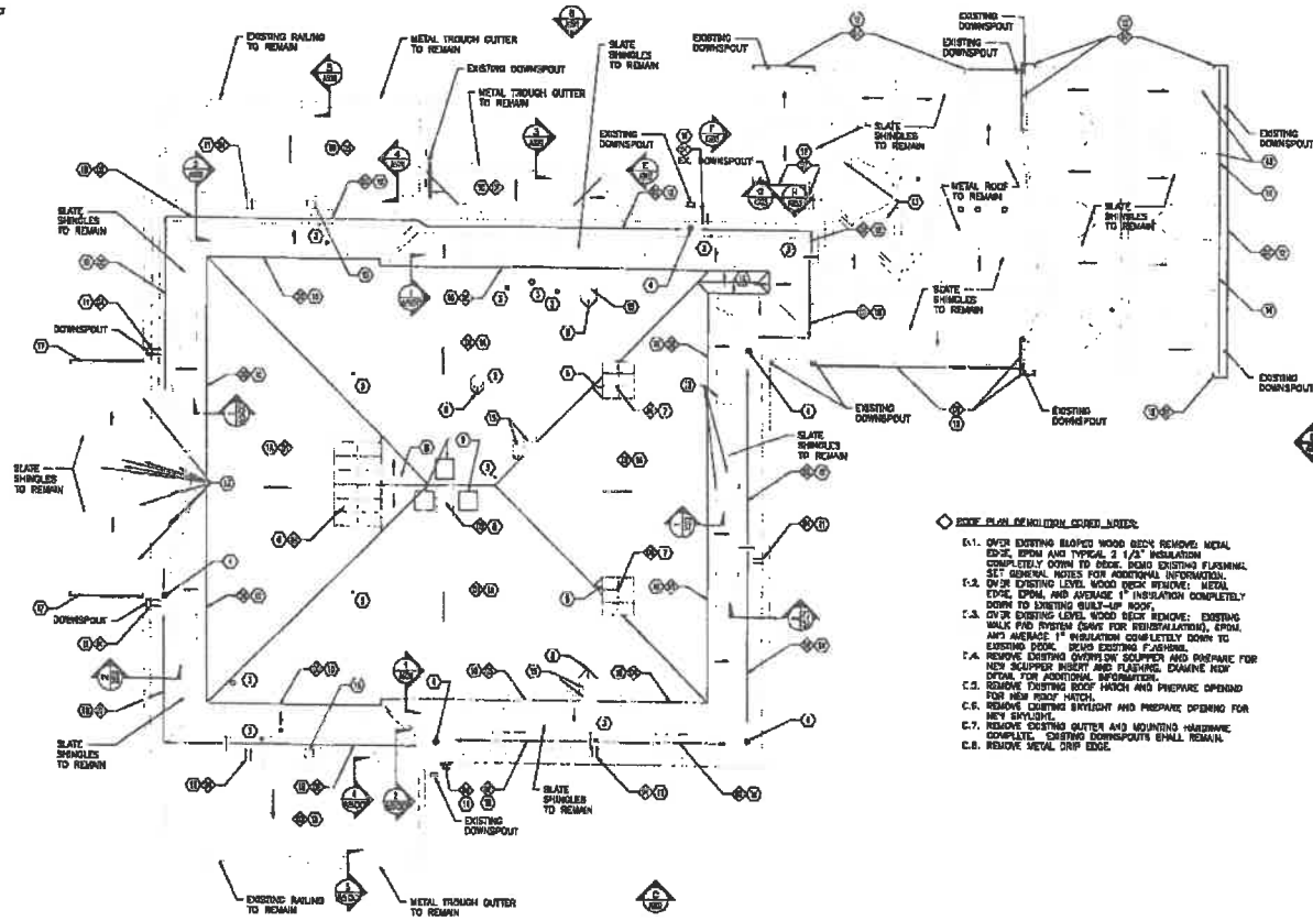
ROOF DEMO AND CONSTRUCTION PLAN SCALE: 1/8" = 1'-0"
