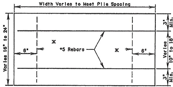
ELEVATION VIEW
