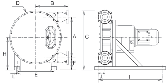
ABN25 - ABN100 Pump
