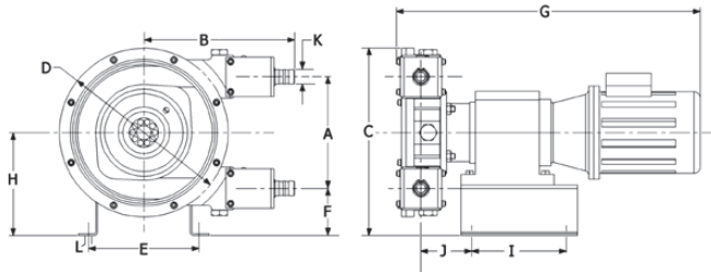
ABN10 - ABN20 Pump
