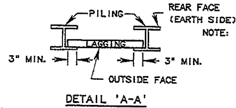
TYPICAL DETAILS FOR CONCRETE LAGGING
