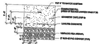
3 TELE/DATE TRENCH SECTION #2 DRAWINGS NOT SCALEABLE
