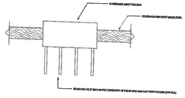
6 IN-GROUND BOX ENLARGED DETAIL (PLAN) DRAWINGS NOT SCALEABLE
