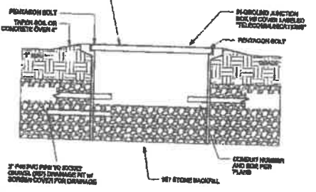
5 IN-GROUND BOX DETAIL DRAWINGS NOT SCALEABLE
