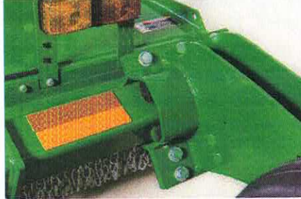
Rubber tubes absorb axle movement
