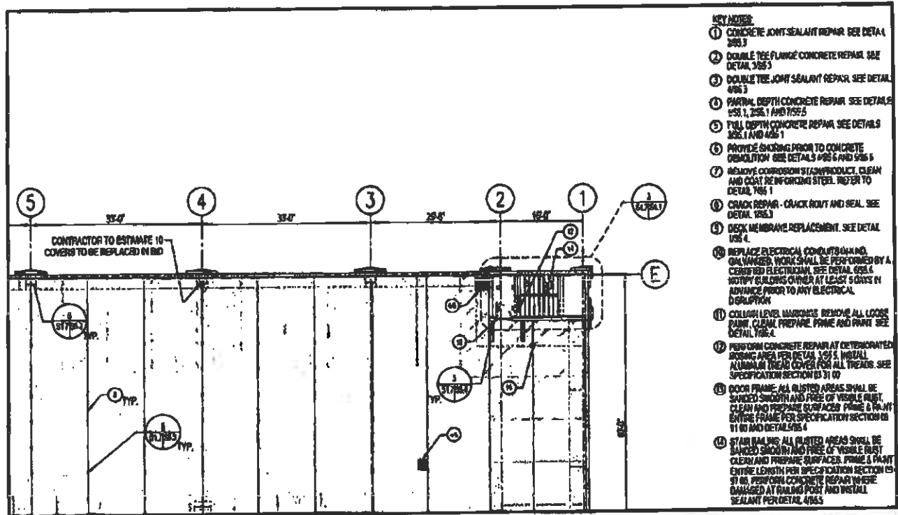
Figure 2 - Partial Deck View, Building 13 Parking Garage Rehabilitation
