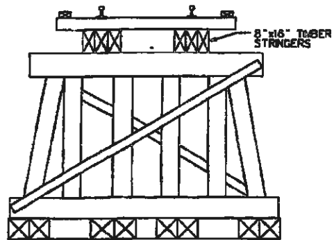
TIMBER FRAME BENT 5
