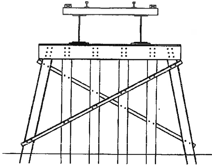
SPAN 16-31: W36X230
