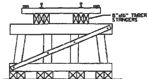
TIMBER FRAME BENT 2
