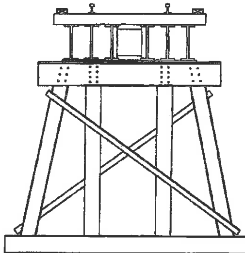
SPAN 35-37: 3-PLY WF26" BEAM
