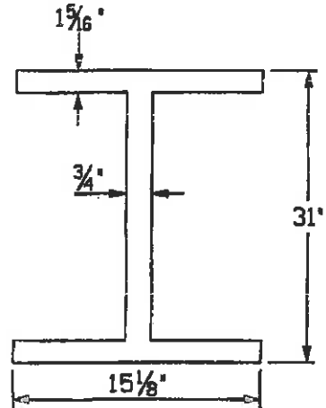
SPAN 32-34: 2-PLY W30X211
