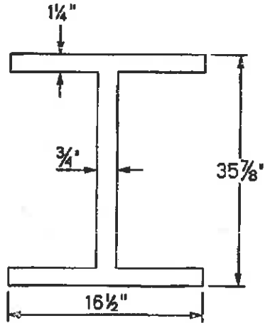
SPAN 16-31: W36X230
