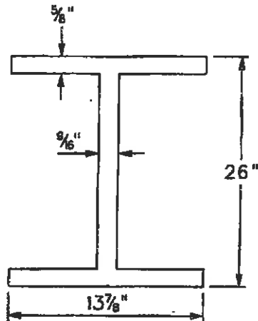
SPAN 35-37: 3 PLY WF26" BEAM
