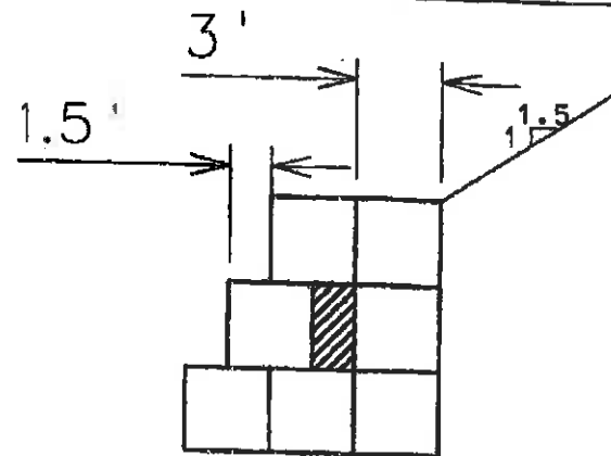
TYPICAL SECTION
