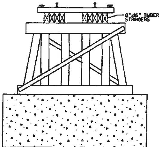
TIMBER FRAME BENTS 3 & 4
