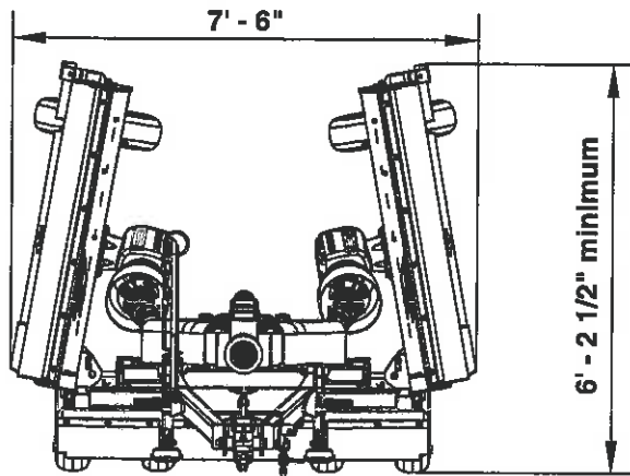
Transport Width With Transport Locks & Deflectors Removed And Cylinders Fully Retracted
