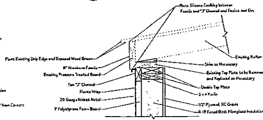
6 Detail "6" Sheet 4/1" = 1'-0"
