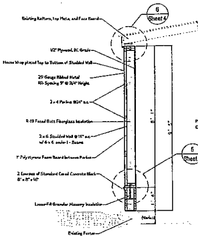
AA Section AA - General Wall Layout Sheet 4/3/8" = 1'-0"
