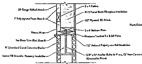
5 Detail "5" Sheet 4/1" = 1'-0"
