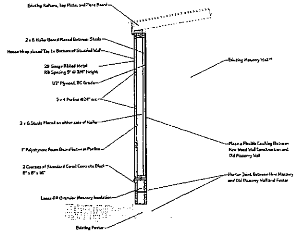
CC Section CC - Masonry Partition Connectors Sheet 4/3/8" = 1'-0"
