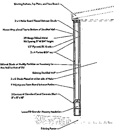
BB Section BB - Studded Partition Connectors Sheet 4/3/8" = 1'-0"
