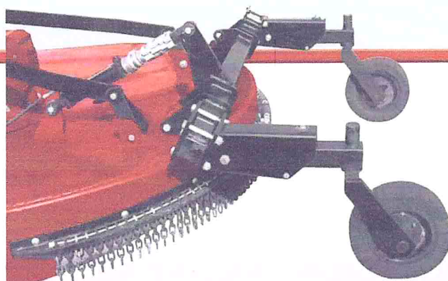
327 Lift Type Cushioned Axle
