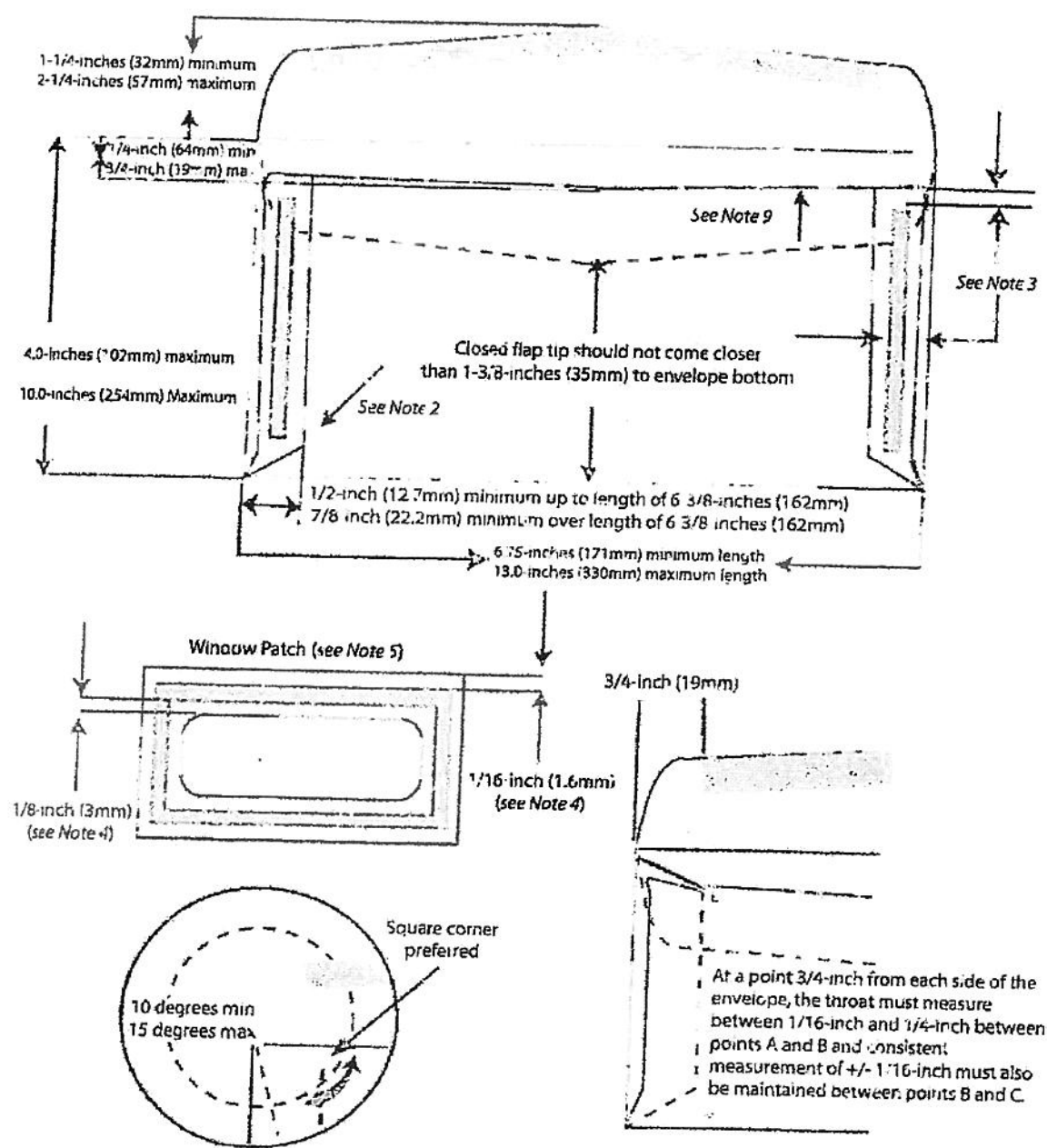
Figure 1-9: Side Seam Envelope Diagram
