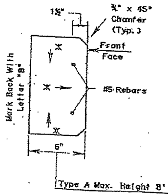
END VIEW
