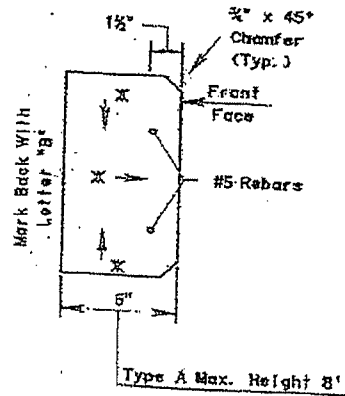
END VIEW
