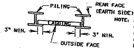
DETAIL "A-A"
