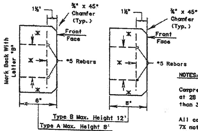
END VIEW
