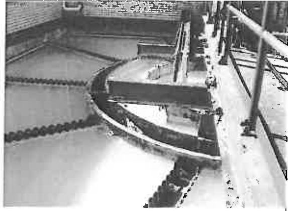
Upflow Clarifier Prior to Replacement
