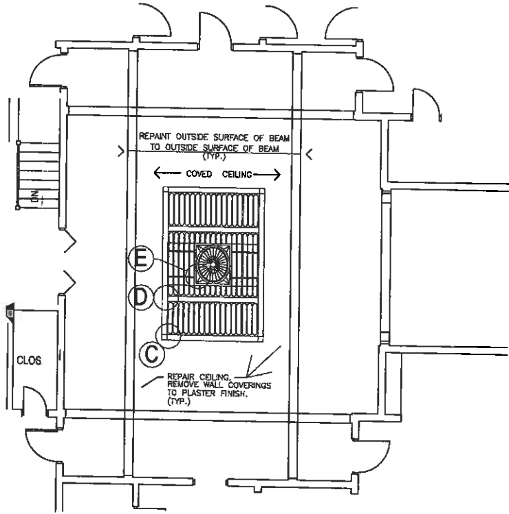
Reflected Ceiling Plan at Coved Ceiling
