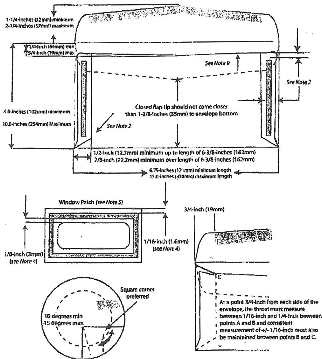
Figure 1-9: Side Seam Envelope Diagram
