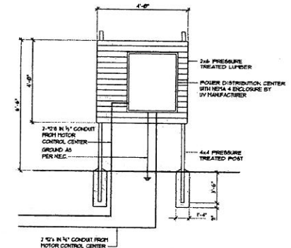
POWER DISTRIBUTION CONTROL SCHEMATIC SCALE: NONE
