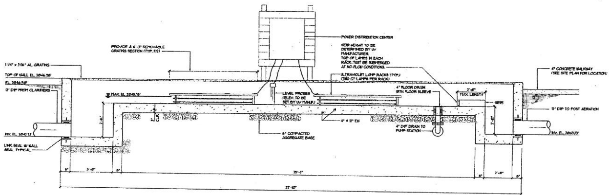
ULTRAVIOLET DISINFECTION SYSTEM SECTION SCALE: 3/4\"/>
