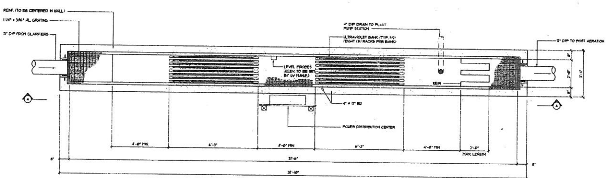
ULTRAVIOLET DISINFECTION SYSTEM PLAN SCALE: 1/4\"/>
