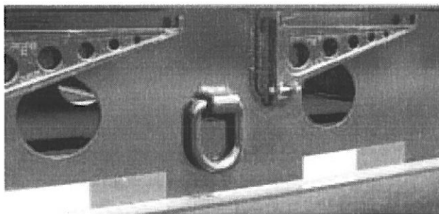
Flat style lash rings and outriggers
