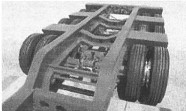
Rear section with spring suspension.
