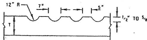
SECTION C-C (MILLED RUMBLE STRIP)
