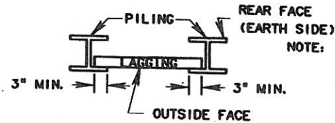
DETAIL 'A-A'
