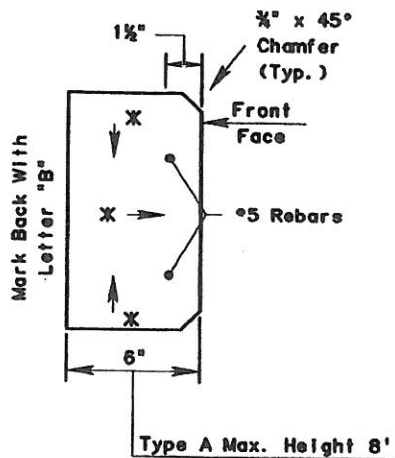
END VIEW
