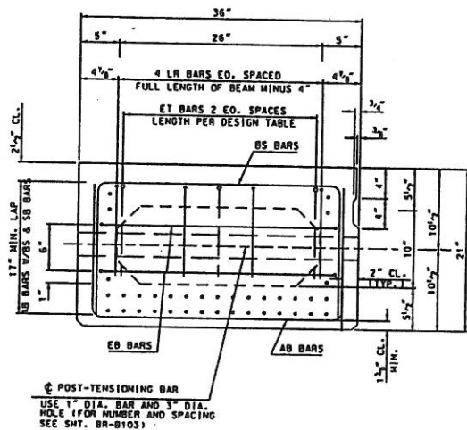
SECTION A-A TYPICAL BEAM REINFORCEMENT
