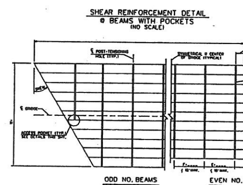
PLAN VIEW-SKEWED BRIDGE > 20° POST-TENSIONING BAR SPACING (NO SCALE)
