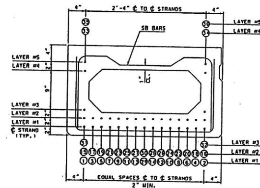
SECTION B-B TYPICAL BEAM PRESTRESSING
