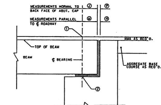
CONTROL ELEVATIONS & BEARING DIMENSIONS ALONG C ROADWAY DETAIL "A"
