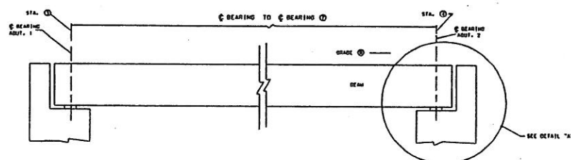
CONTROL ELEVATIONS & BEARING DIMENSIONS ALONG C ROADWAY DETAIL "A"
