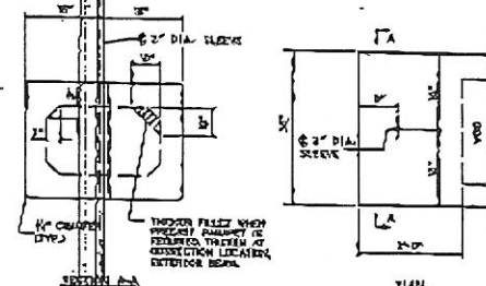
END BLOCK DETAILS
