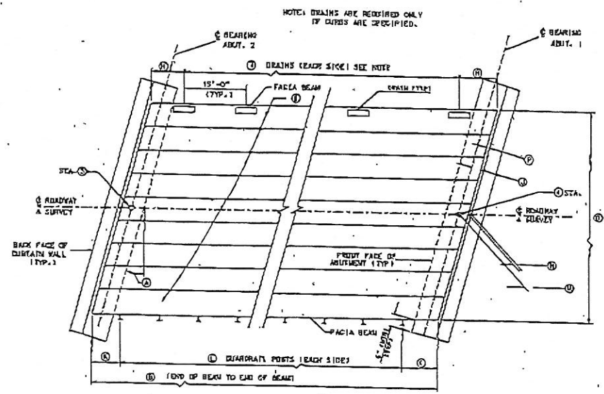
SUPERSTRUCTURE LAYOUT PLAN
