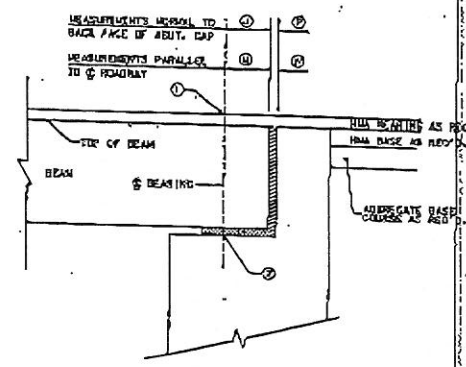
CONTROL ELEVATIONS & BEARING DIMENSIONS ALONG & ROADWAY DETAIL "A"
