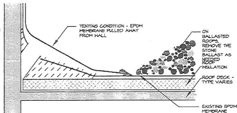
A WALL BASE FLASHING (BRIDGING CONDITION) - STEP 1
