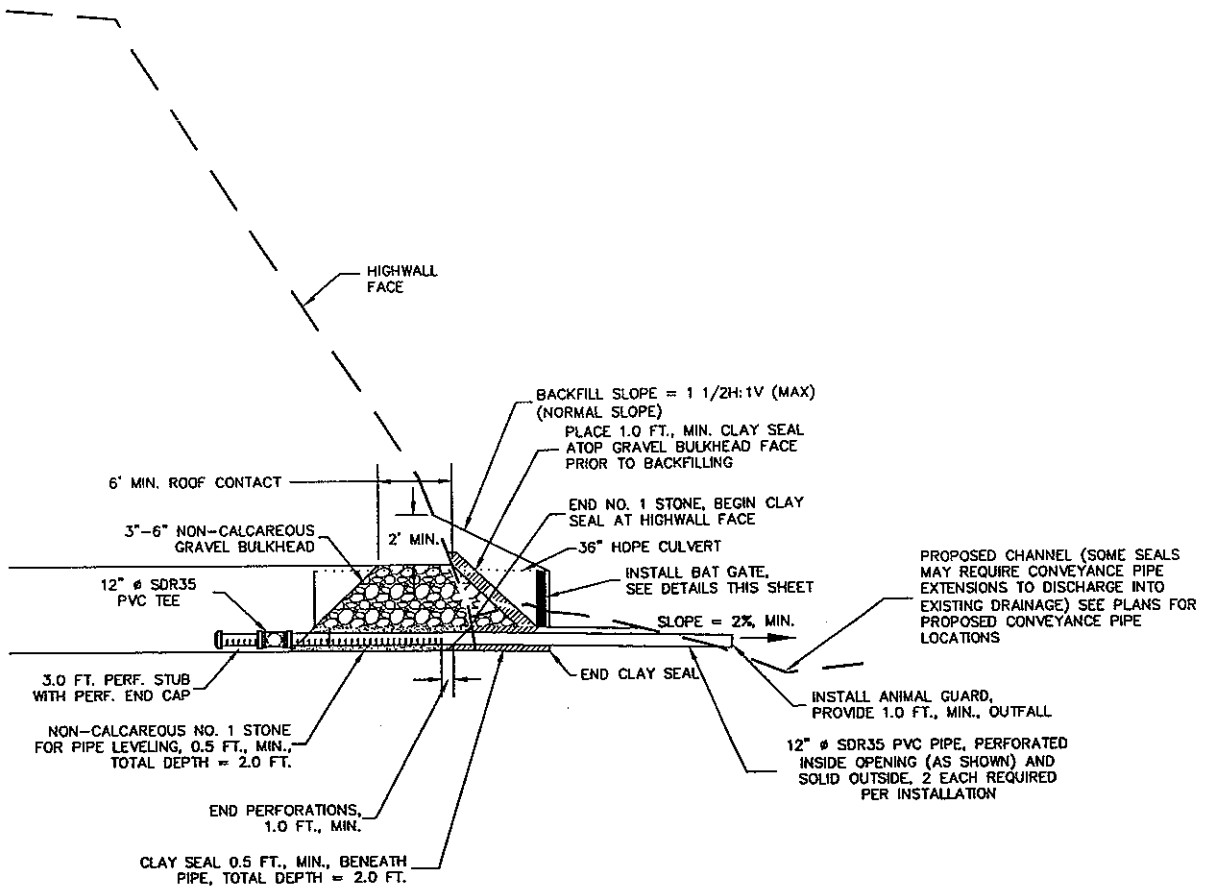
TYPICAL SECTION
