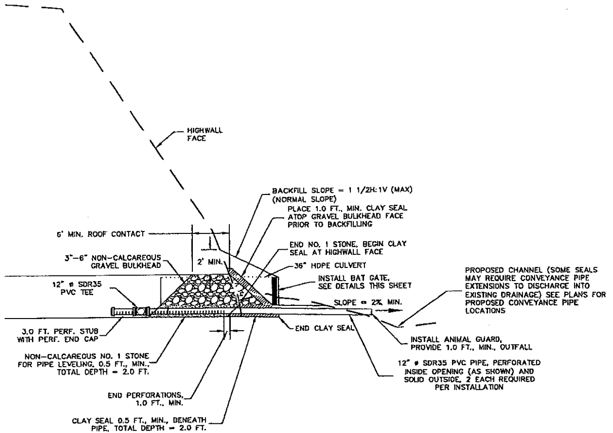
TYPICAL SECTION
