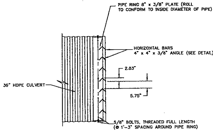
TYPICAL SECTION
