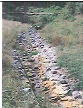
NIXON RUN AMD: Wet Mine Seal outlet pipes and receiving ditch.
