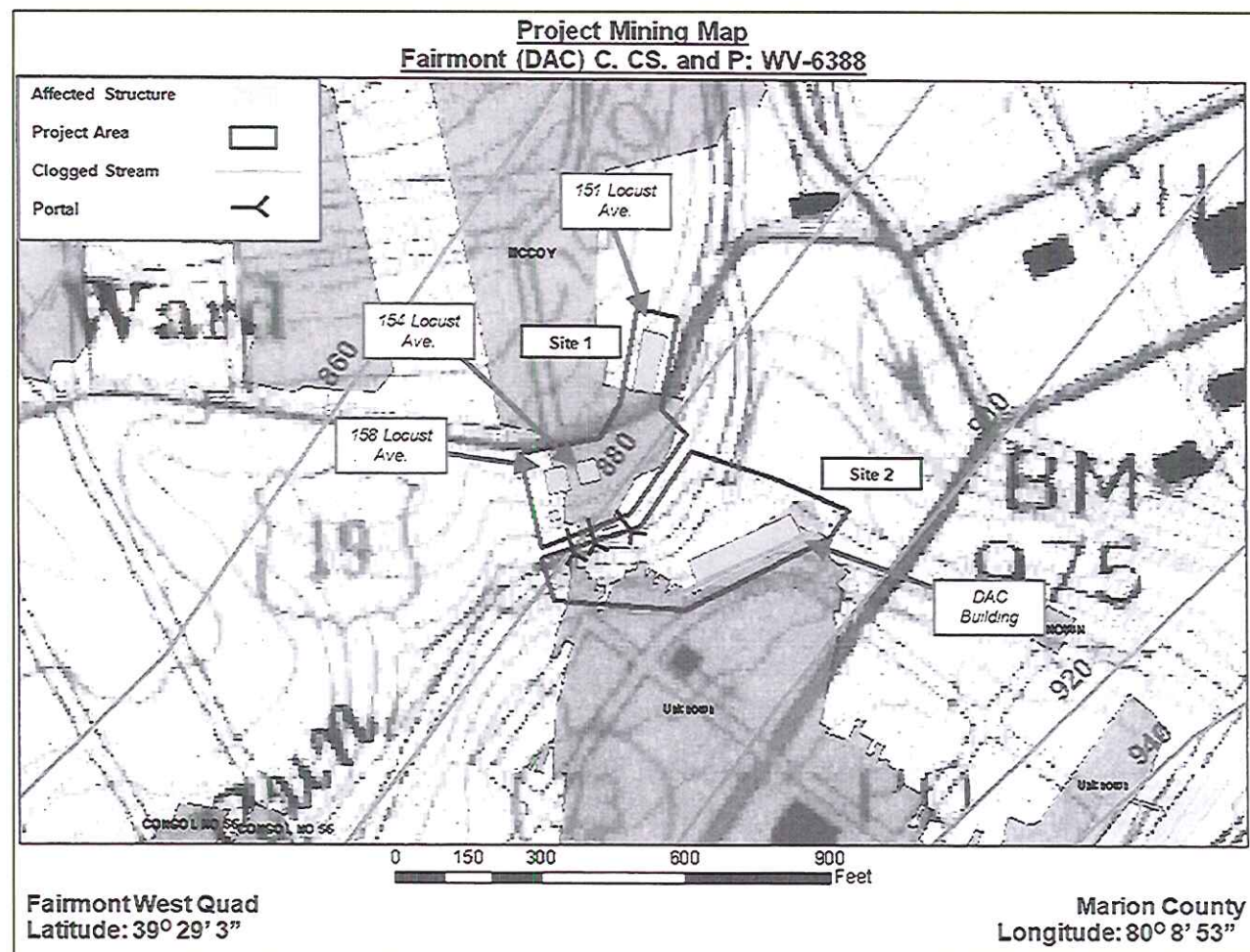
Pittsburgh Coal Mined Out Areas and Structure Contour Map - Fairmont (DAC), S, CS, P
