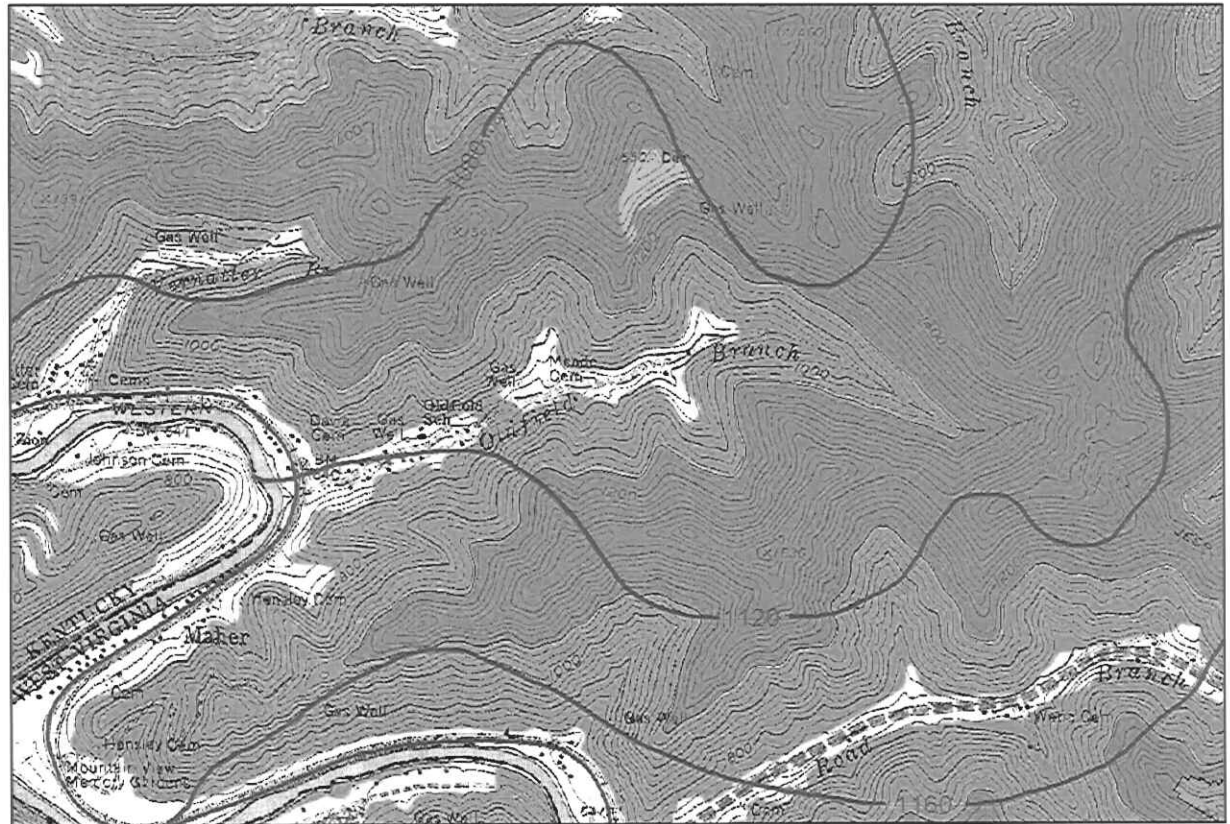
Coalburg Seam Structure Contour Map - Oldfield Branch
