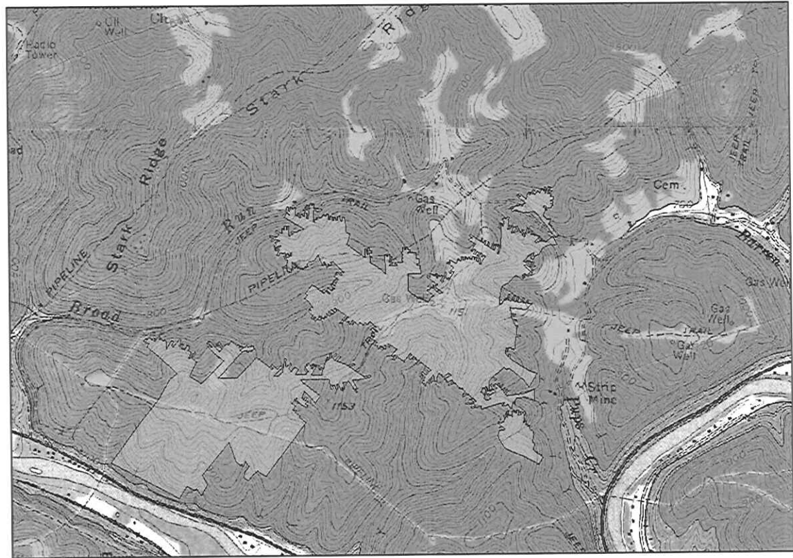
No. 5 Block Mined Out Area and Structure Contour Map – Broad Run Site
