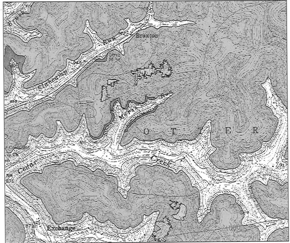
Pittsburgh Coal Structure Contour Map and Mined Out Area – Marsh Run Portals
