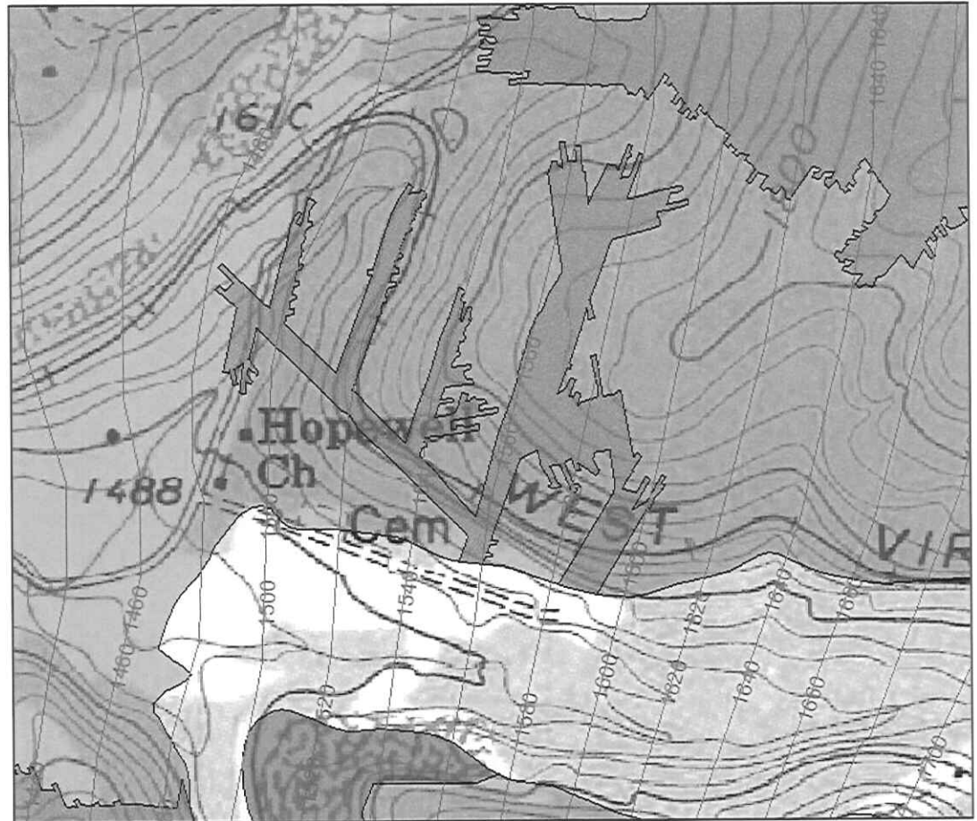
Upper Freeport Coal Mined out Areas and Structure Contour Map – Hopewell Church
