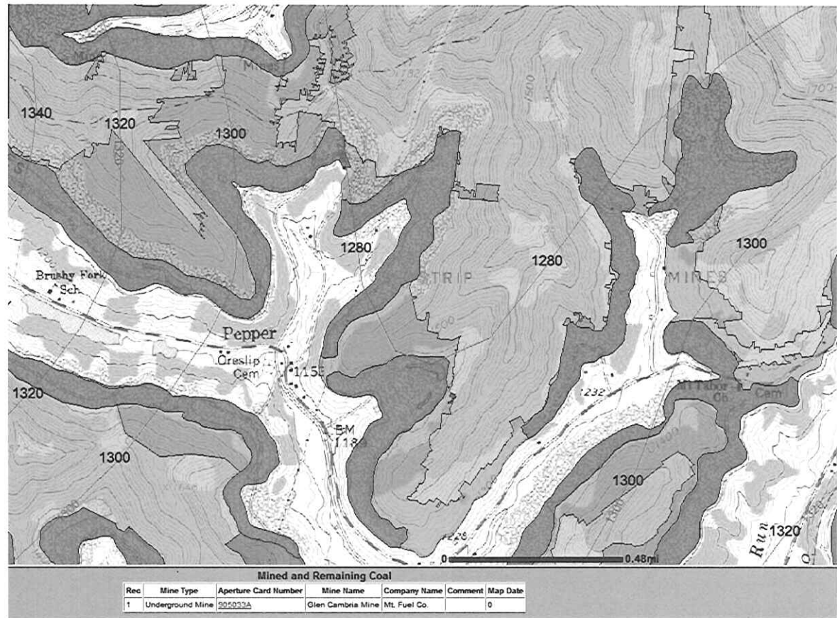
Pittsburgh Coal Mined Out Areas and Structure Contour Map – Pepper Portal
