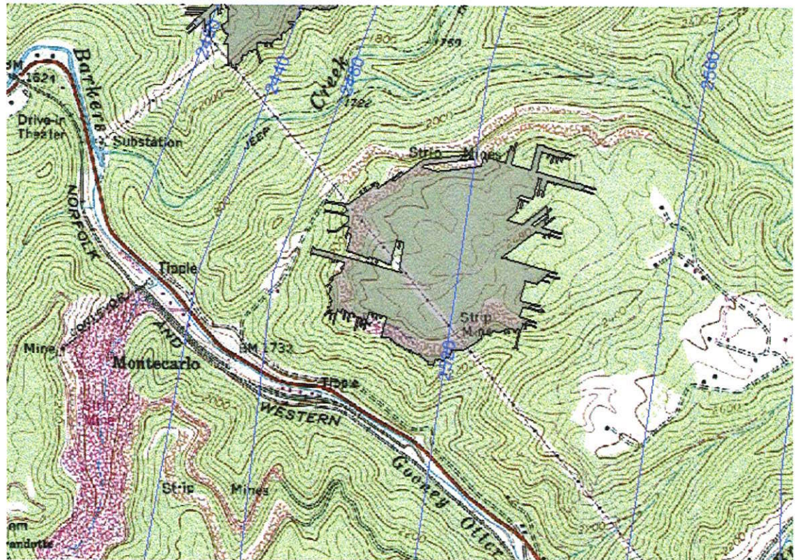
Structure Contour Map and Mined Out Area - Montecarlo Complex
