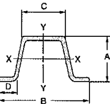
Sign Post and Base Post Weight - 3.00 lbs/ft
