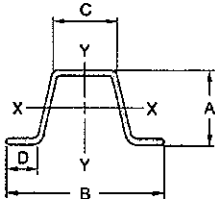
Sign Post and Base Post Weight - 2.00 lbs/ft
